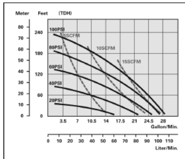
Performance Graphs based on 305 mm flooded suction, with water at ambient temperature
