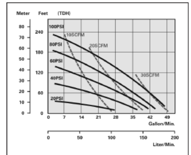
Performance Graphs based on 305 mm flooded suction, with water at ambient temperature
